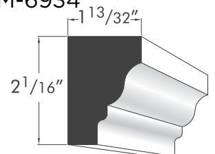
Rams Crown AZM-6934
