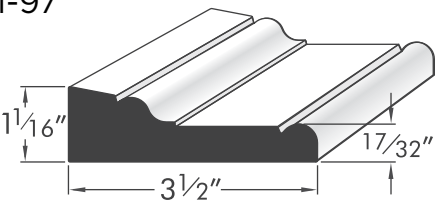
Adams Casing AZM-97
