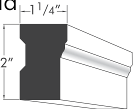
Rake Moulding AZM-287
