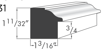
Brick Mould AZM-180
