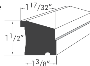
Sub Sill Nose AZM-6933
