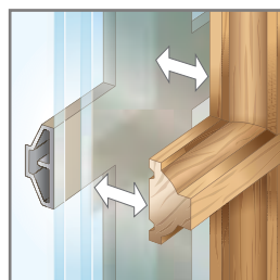
SHOWN WITH COLONIAL PROFILE AND OPTIONAL FIXED EXTERIOR GRILLE
