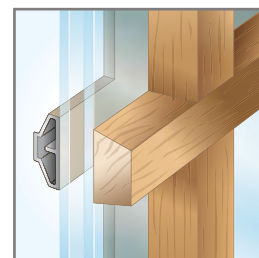
SHOWN WITH CONTEMPORARY PROFILE
